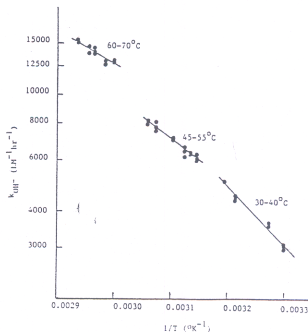
Fig. 2. Semilogarithmic Arrhenius plots of k_{OH^-} vs 1/T obtained for the hydroxyl ion-catalyzed aspirin hydrolysis in the 30–40, 45–55, and 60–70°C temperature ranges.
