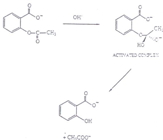
Scheme II. Hydroxyl ion-catalyzed aspirin hydrolysis.
