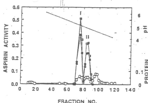
Fig. 2. Elution from a chromatofocusing column leading to separation of esterases I and II. Key: hydrolytic activity for acetylsalicylate (■) and 4-nitrophenylacetate (□); protein (○). The dashed line indicates pH of the eluate.
