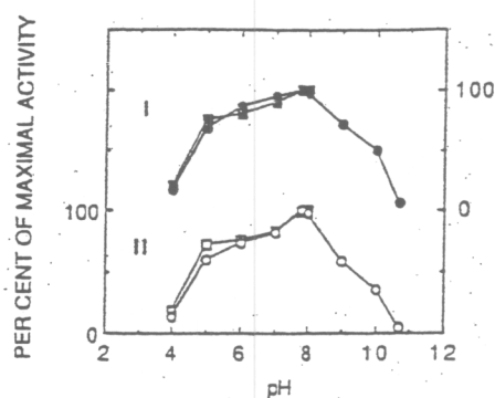
Fig. 3. Activity as a function of pH for esterase I (upper curves) and esterase II (lower curves) using acetylsalicylate (circles) and 4-nitrophenylacetate (squares) as substrates.
