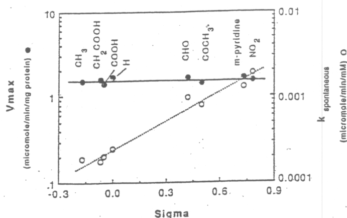
Fig. 4. Effect of substituents on enzymatic (●) and spontaneous (○) hydrolysis of phenylacetates in 50 mM Bicine at pH 8.0. All substitutions are at the 4-position with the exception of pyridine at the 3-position. Values for \sigma are from Ref. 27.
