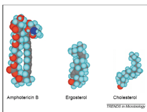
Fig. 3. The polyene antifungal agent, amphotericin B, ergosterol and cholesterol, visualised in three dimensions. Ergosterol, the sterol found in fungal cell membranes, retains a cylindrical shape in all rotations and binds better to the hydrophobic (right-hand) side of the amphotericin B molecule than does cholesterol, with its sigmoid structure. Cholesterol is the membrane sterol found in mammalian cells; the differential binding affinity of amphotericin B for the two sterols is the basis of its selective antifungal action.
