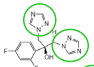
Fluconazole
