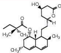
Simvastatine IC50 = 11 nM
