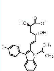
Fluvastatine IC50 = 28 nM
