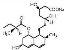
Pravastatine IC50 = 40 nM
