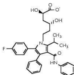
Atorvastatine IC50 = 8 nM
