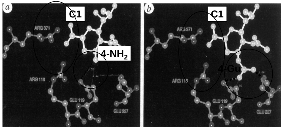
4-deoxy-4-amino ...
