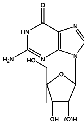
(deoxy)GUANOSINE
