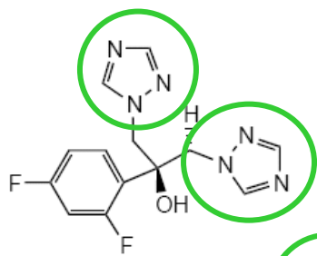
Fluconazole
