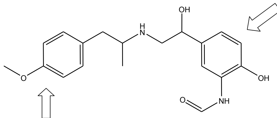
formoterol
