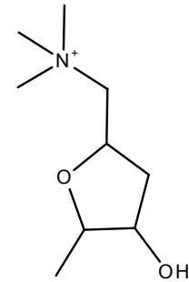
muscarine
