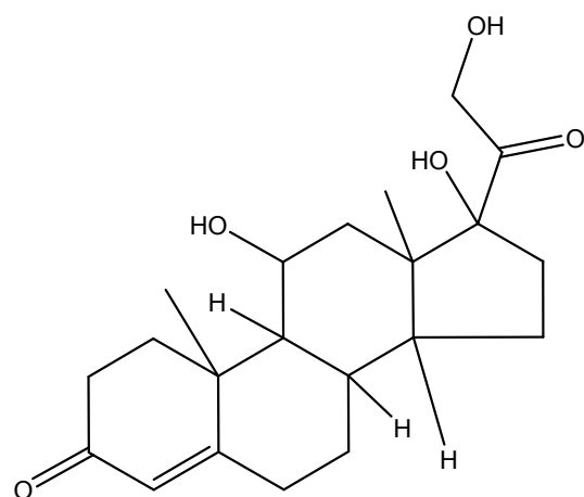
hydrocortisone
