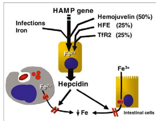
Fig. 3. - Hepcidin and regulation of iron metabolism. Hepcidin is a peptide expressed by gene HAMP in liver cells in response to infection and iron overload. Hemojuvelin, protein 181, and transferrin receptor 2 (TfR2) also contribute to increase hepcidin production. This slows the passage of iron through enterocytes (intestinal absorption) and the release of iron from macrophages. In these cells iron stems from the degradation of phagocytosed old red blood cells. Hepcidin has been suggested to exert these effects by internalizing transferrin 1 (TfR1) within cells.
