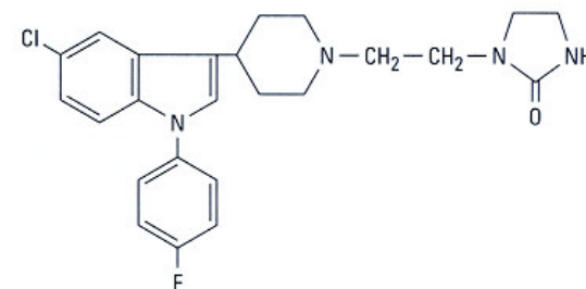
Sertindole
