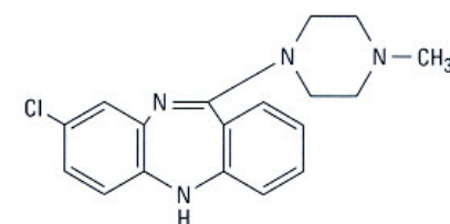
Clozapine
