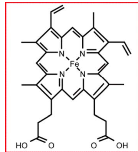
myoglobin hemoglobin
