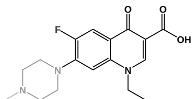
pefloxacin e
