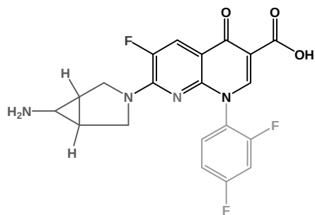
trovafloxacin
