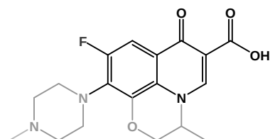
ofloxacin e
