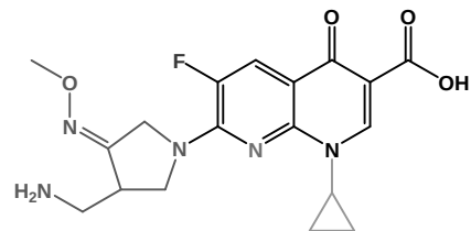
gemifloxacin
