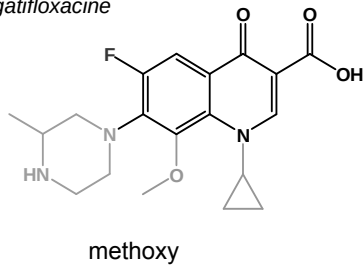
gatifloxacin
