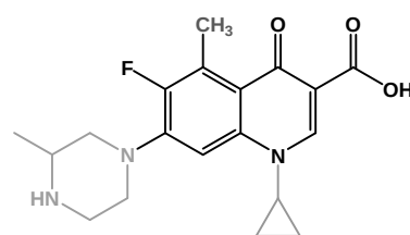
grepafloxacin
