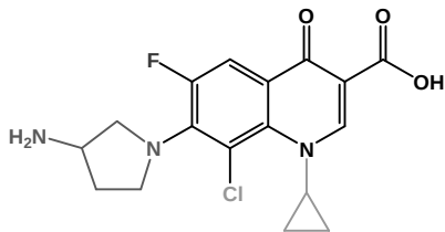
trovafloxacin
