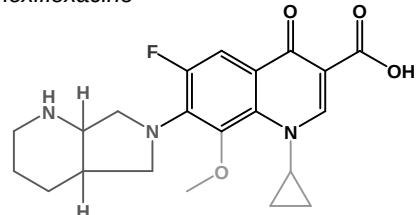
gemifloxacin
