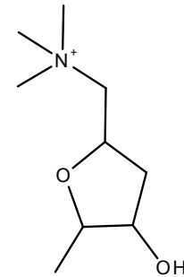
muscarine
