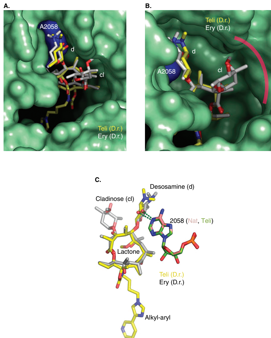
Figure 1. Comparison of the mode of interaction of erythromycin A and telithromycin with 23S rRNA (see also [3,148]). A. View onto the ribosomal exit tunnel entrance of the 50S model from Deinococcus radiodurans (D.r., D50S), 23S rRNA is displayed as mint surface (Ade2058 is marked in blue, E. coli numbering used for figures). Macrolides like erythromycin A (Ery, grey) and ketolides like telithromycin (Teli, yellow) inhibit translation by blocking the ribosomal exit tunnel [3,149] and thus prevent the nascent peptide chain to move forward, which leads to translation arrest in most cases. B. Zoom and slightly different orientation of A . Methylation or mutation A- > G of Ade2058 has as consequence that the hydrogen bond of the desosamine-moiety (d) of the macrolides/ketolides to 2058 (see also C ) is not possible and that the antibiotic needs to be shifted away from A2058. The cladinose moiety (cl), close to the tunnel wall (pink line) restricts possible positionings of the macrolides (Ery, grey) for alternative binding to ribosomes with mutated or methylated 2058. Ketolides (Teli, yellow) lacking the cladinose have much more room for an alternative positioning which, together with the additional, stabilizing binding of their alkyl-aryl side chain, can overcome A2058 methylation/mutations in many bacteria. C. Macrolides and ketolides bind in similar mode to the ribosome. The lactone ring overlaps with high agreement and the hydrogen bonds (green dotted) between Ade2058 (of 23S; Nat, native, position in the absence of antibiotic; teli, position in the presence of telithromycin) and the desosamine-moiety differ only slightly for telithromycin (yellow, 2058 in green) and erythromycin A (grey, 2058 in pink) in D50S.
