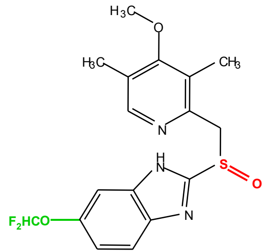
pantoprazole
