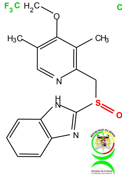
lansoprazole
