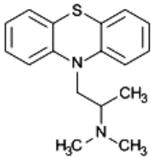
Promethazine
